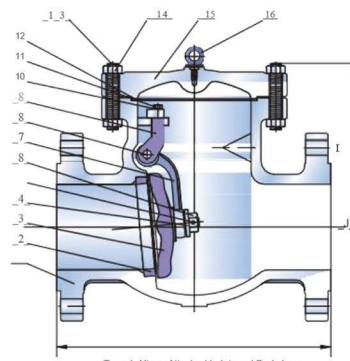
Type 1: Hinge Attached to Internal Body Lug
